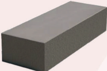
BRADSTONE PAVER SIZE-275X100X60mm
